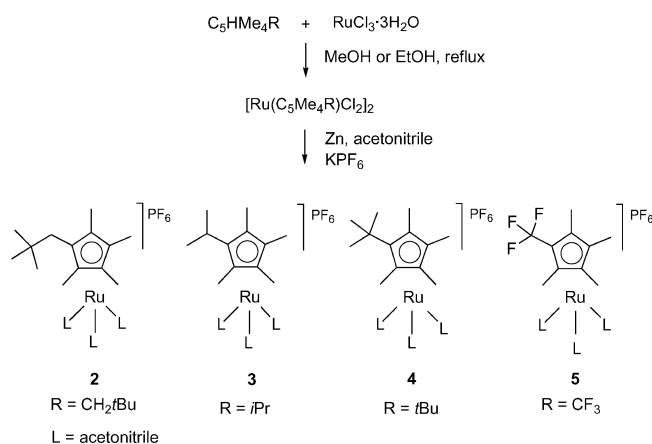
Scheme 1. Synthesis of [\text{Ru}(\eta^5\text{-C}_5\text{Me}_4\text{R})(\text{MeCN})_3][\text{PF}_6] complexes 2–5 .
