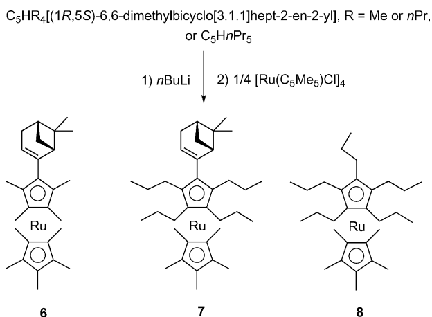
Scheme 2. Synthesis of the new fully substituted ruthenocenes 6–8 .
